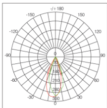
SL368-3W-3000K-40°
